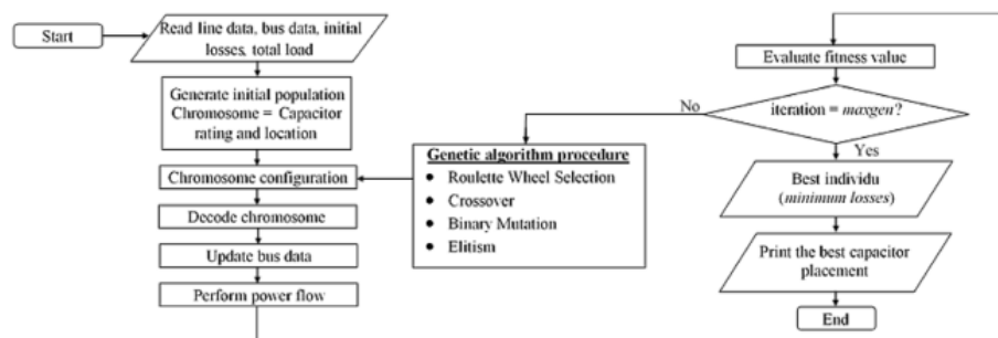
Fig. 1. Flowchart of capacitor placement with genetic algorithm.
